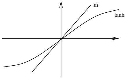
Figure 44: \tanh(Jqm\beta) for Jq\beta < 1
